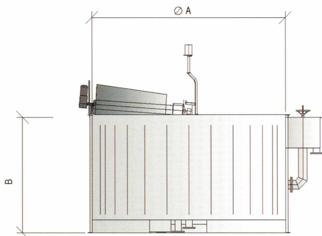
SDC 49 - Biological sludge thickening (municipal)
