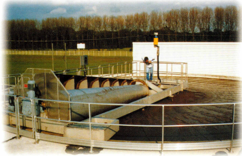
SDC 49 - Biological sludge thickening (municipal)
