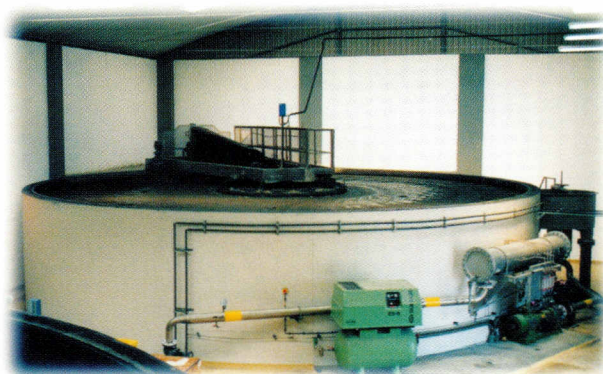
SDC 36 - Concentrating sludge from biofilter backwashing
